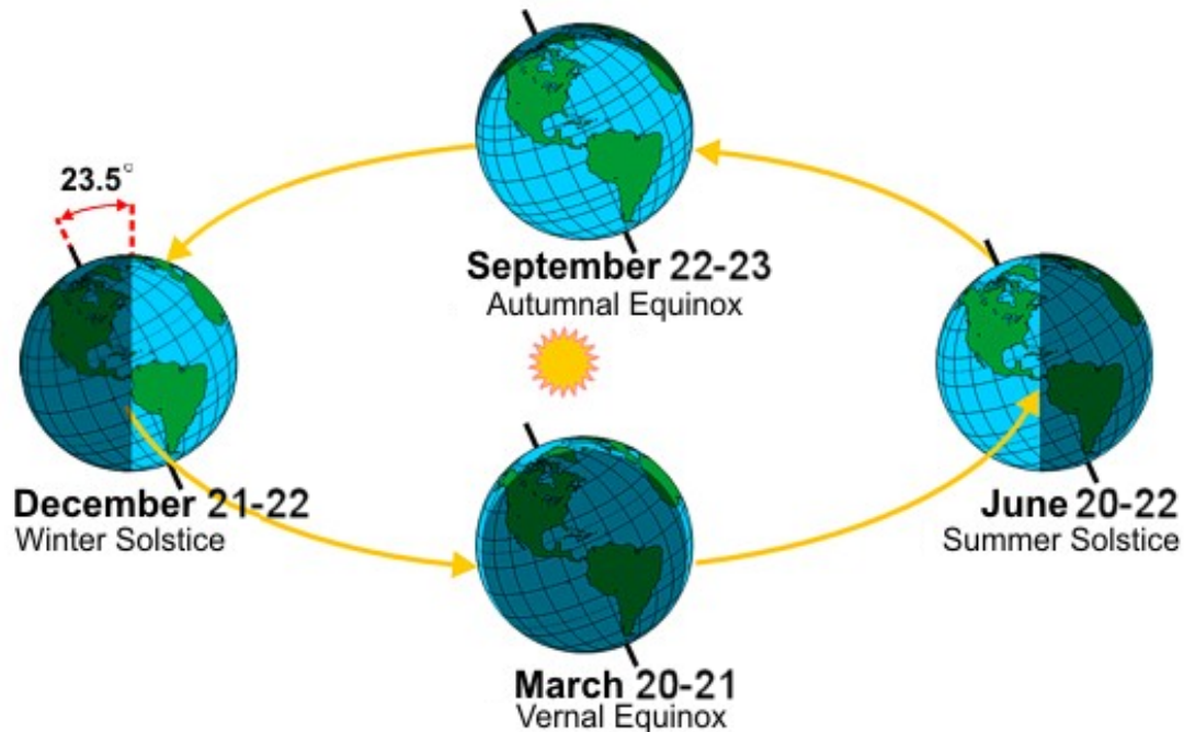
Figure 5.27 Seasons Diagram, Note the Tilt and Circle of Illumination for Each Season. Image is in the public domain.
