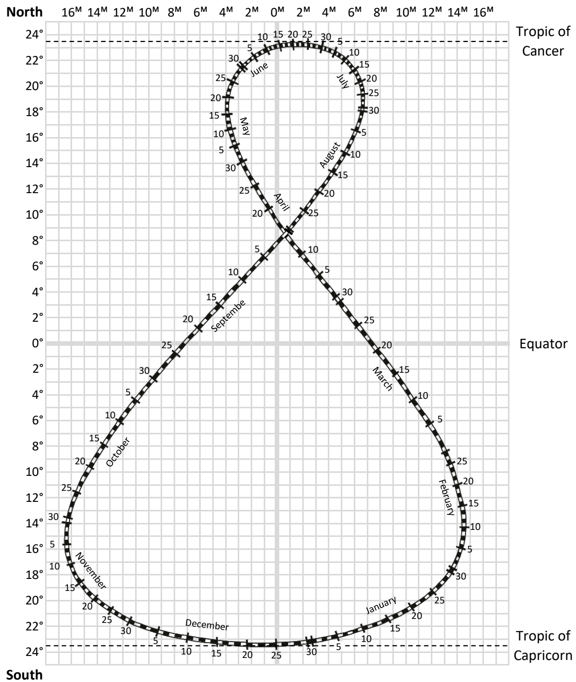
Figure 5.30 The Analemma. Image by Jeremy Patrich is used under a CC-BY-4.0 license.
