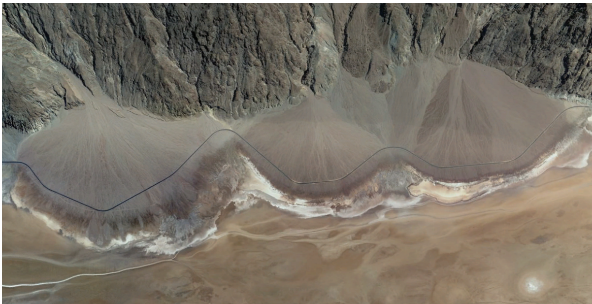
Figure 18.126 A Collection of Alluvial Fans are Called Bajadas, Death Valley National Park, California. Used under Google Earth reproduction guidelines
