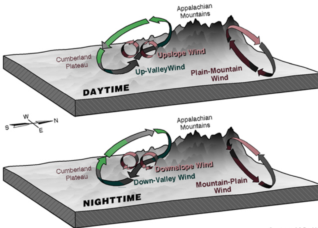
Figure 6.6 Mountain & Valley Breezes. Image is in the public domain.
