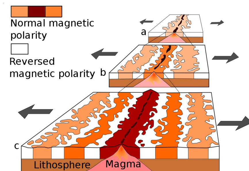
Figure 13.8 The Ocean Floor Shows Patterns of Magnetic Variation That is not Random, This is an Example of the Magnetic Stripping. Image is in the public domain.
