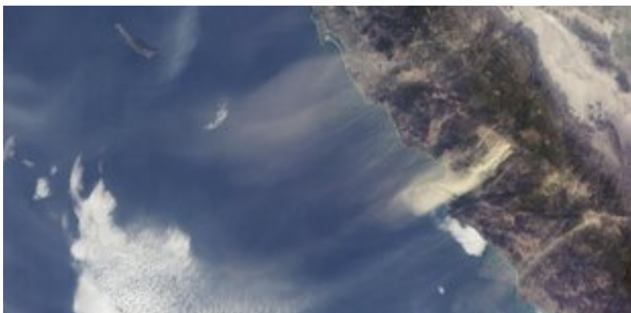
Figure 6.9 The Santa Ana Winds-- Note the Direction of Flow Being Eastward.
