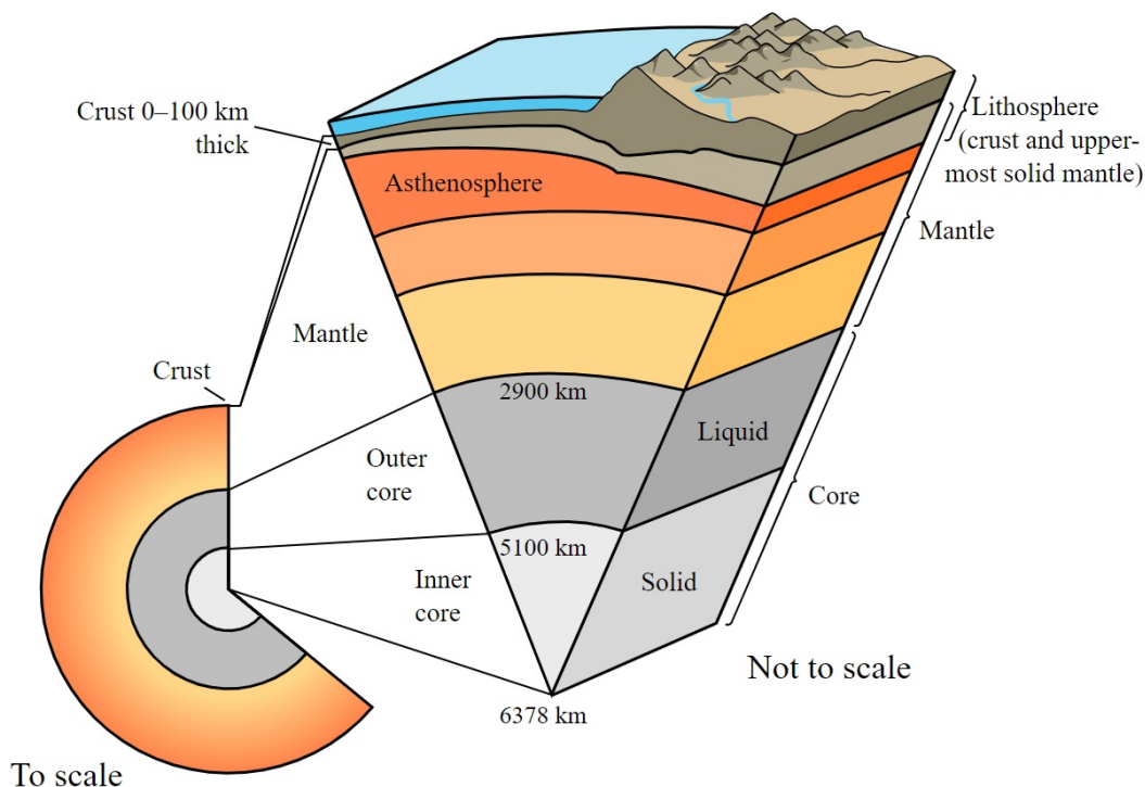
Figure 13.4 A Slice of Earth-- Exposing the Structure & Composition. Image is in the public domain.
