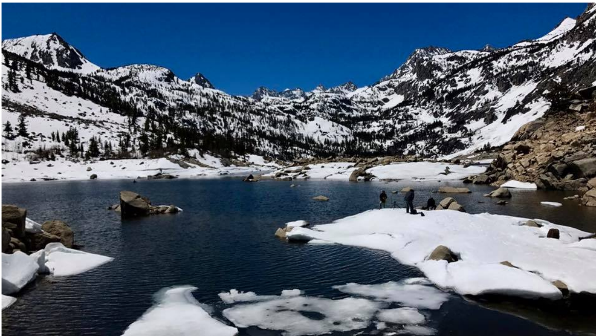
Figure 19.146 Note the Cirque the Envelops Lake Sabrina, a Glacial Tarn. Image by Jeremy Patrich is used under a CC-BY 4.0 license.
