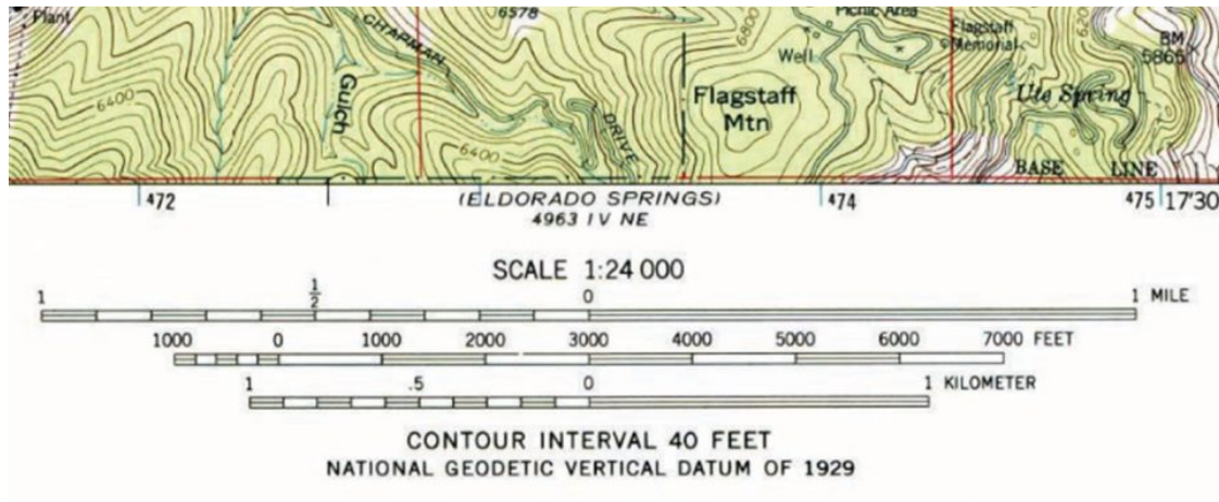
Figure 4.2 Representative Fraction & Scale Bars from a USGS Topographic Map. Image is used under a Creative Commons by-nc-sa 3.0 license.
