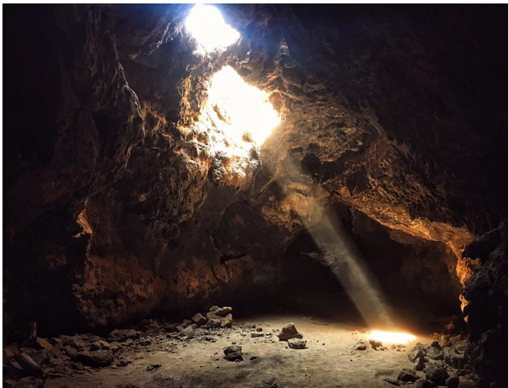
Figure 15.6 Photo from Inside the Mojave Volcanic Tubes. Image by Jeremy Patrich is used under a CC-BY 4.0 license.
